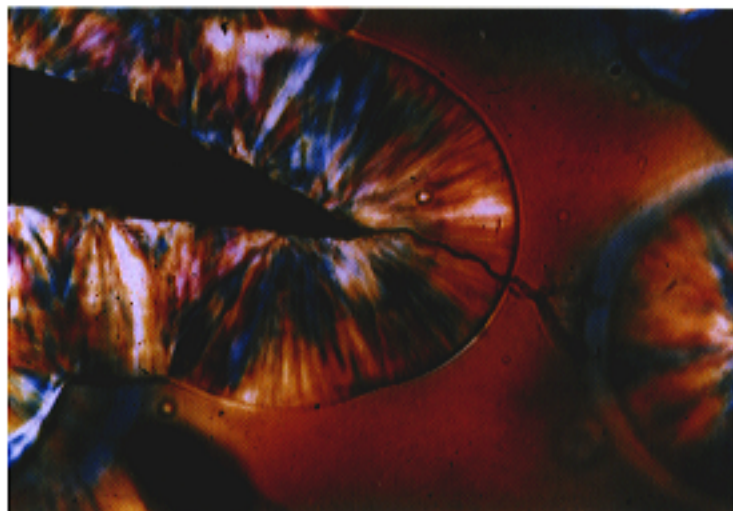
The tree shape in polypropylene spherulite
